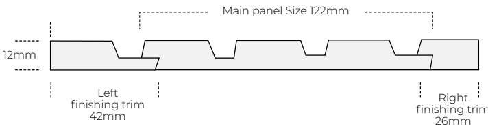
Panel and finishing trim dimensions
